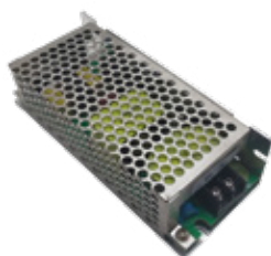
900259 320W IN 100~240V | OUT 380V 0,83A SIZE: 14,3X5,9X3,9cm
