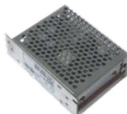
900437 60W IN 100~240V | OUT 12V 5A SIZE: 11X7,9X3,5cm
