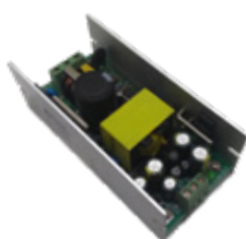
901072 150W IN 100~240V | OUT 12V 1A / 28V 5A SIZE: 12,1X5,7X3,9cm
